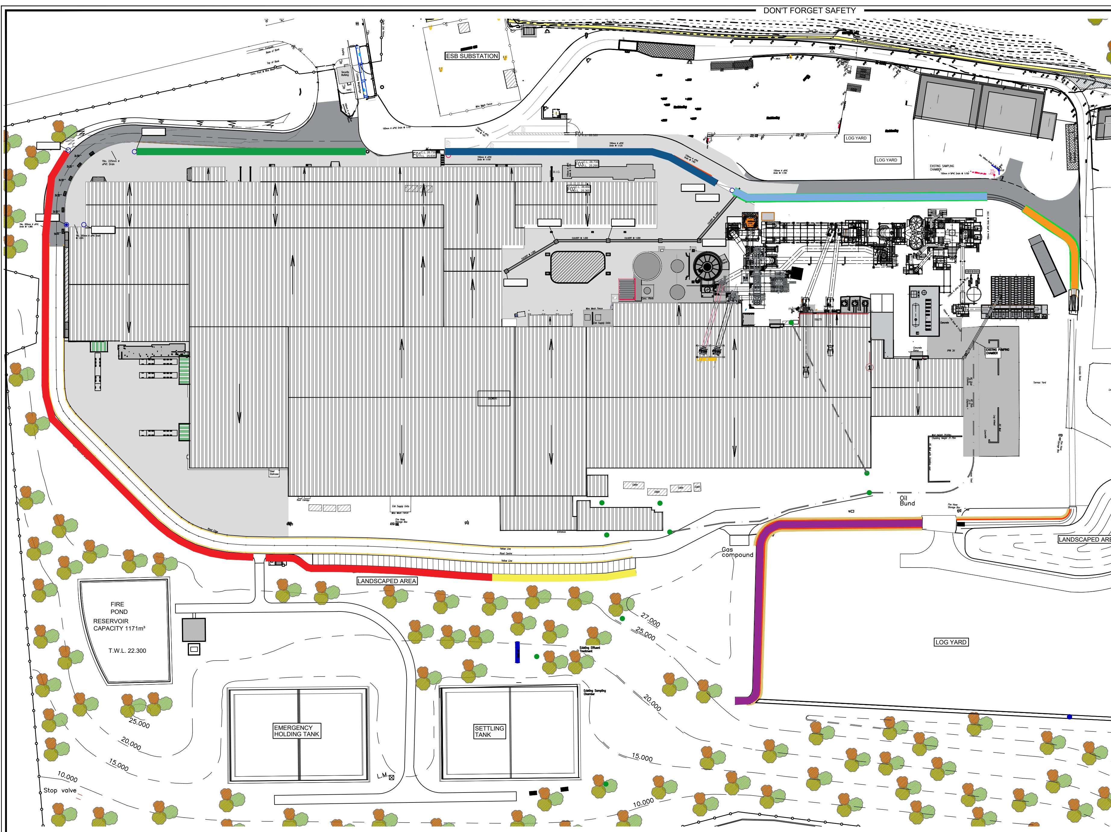
PROPOSED WORK TO EXISTING DRAIN CHANNEL LAYOUT A1 SCALE 1:1000 A3 SCALE 1:2000
