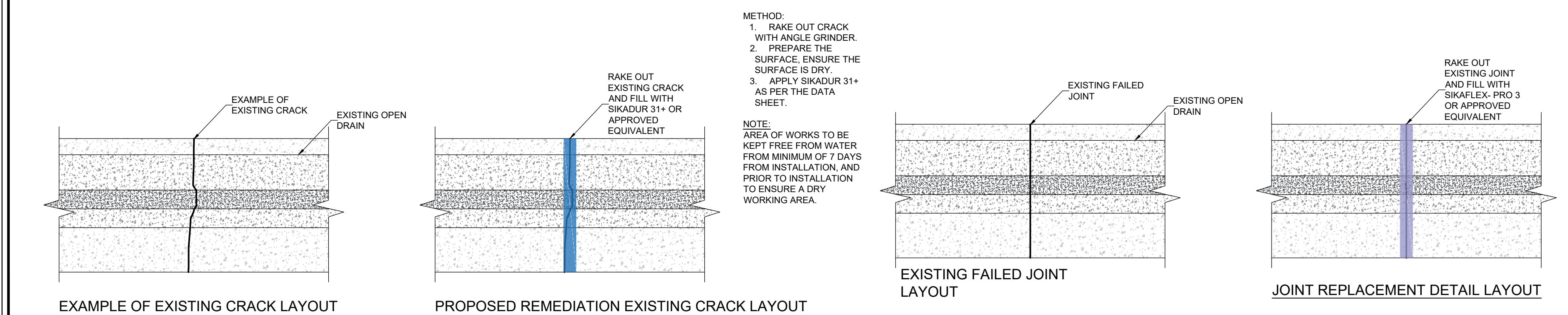
CRACKS REMEDIATION DETAIL Scale A1 1:25 Scale A3 1:50 NOTE: THE CONTRACTOR IS TO ALLOW FOR THE REMOVAL & DISPOSAL OF MOSS AND ANY OTHER DEBRIS FOUND WITHIN THE OPEN CHANNEL DURING THE WORKS. CONTRACTOR MUST ENSURE NO FOREIGN MATERIAL FLOWS DOWNSTREAM FROM THE WORKS.
