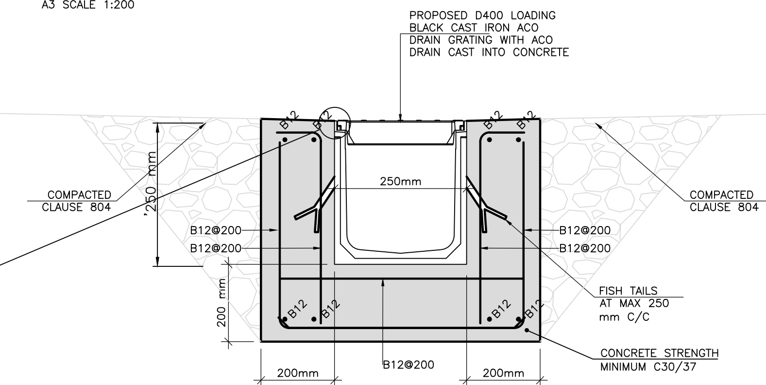
DETAIL 1 ACO DRAIN
