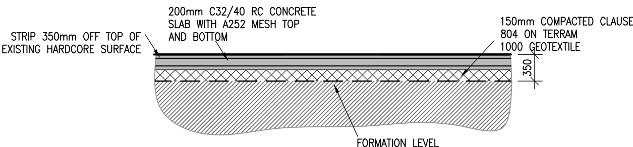
TYPICAL SECTION THROUGH NEW 200mm thk. CONCRETE YARD ROAD SURFACING A1 SCALE 1:50 A3 SCALE 1:100
