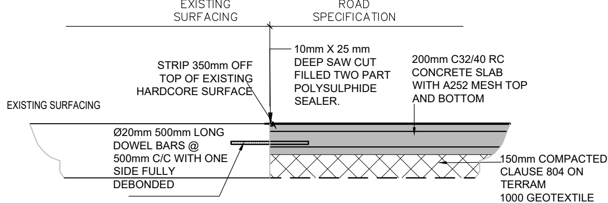
SURFACING INTERFACE DETAIL (ROAD SPEC. TO EXISTING SURFACING) A1 SCALE 1:25 A3 SCALE 1:50 TBC BY CLIENT
