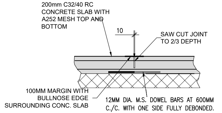
TYPICAL EXPANSION JOINT @ 6m C/C Scale A1 1:25 Scale A3 1:50
