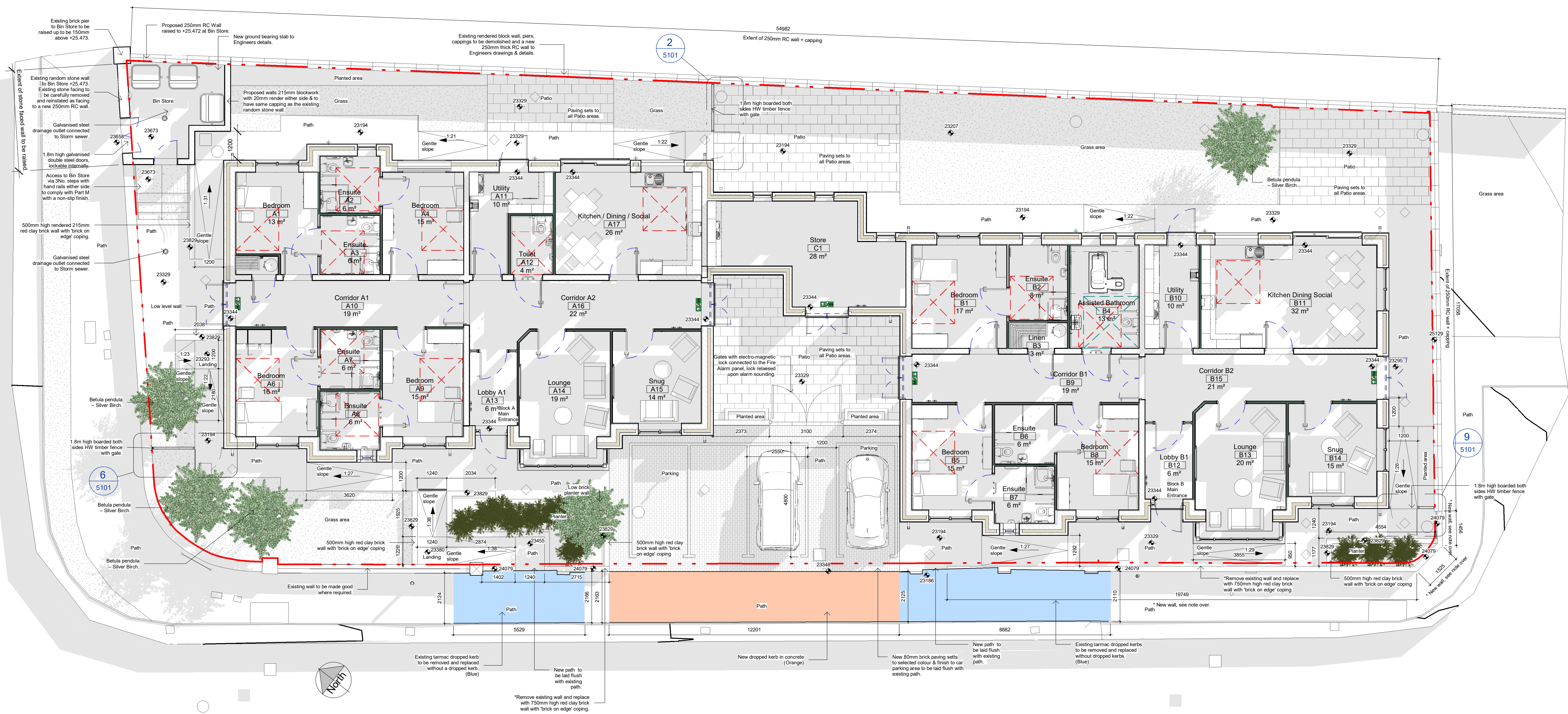
1100 1 1:100 @ A1 Proposed Site Layout Plan
