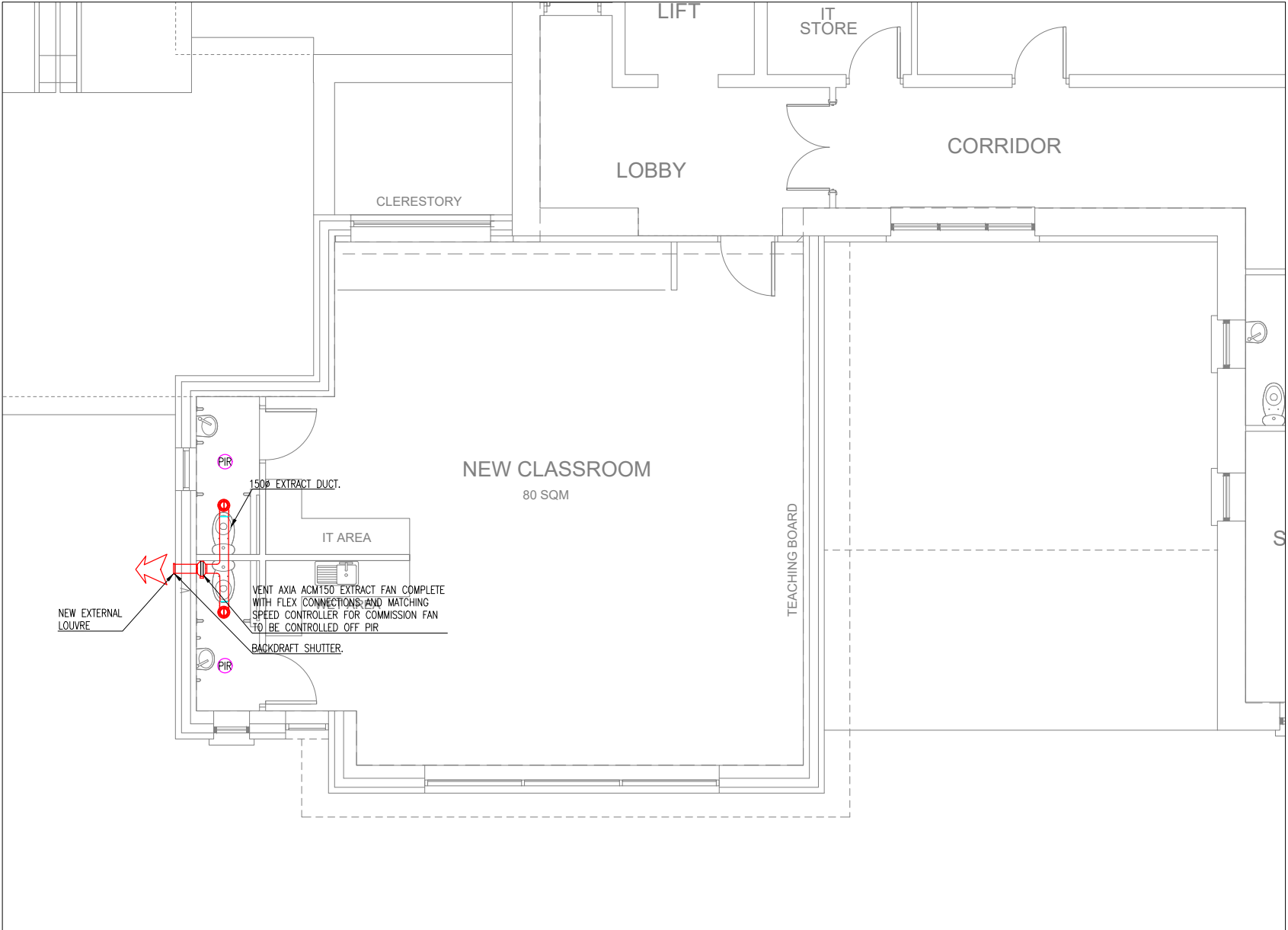
M201 VENTILATION LAYOUT – FIRST FLOOR 01 SCALE 1:50 @ A1 1:100 @ A3
