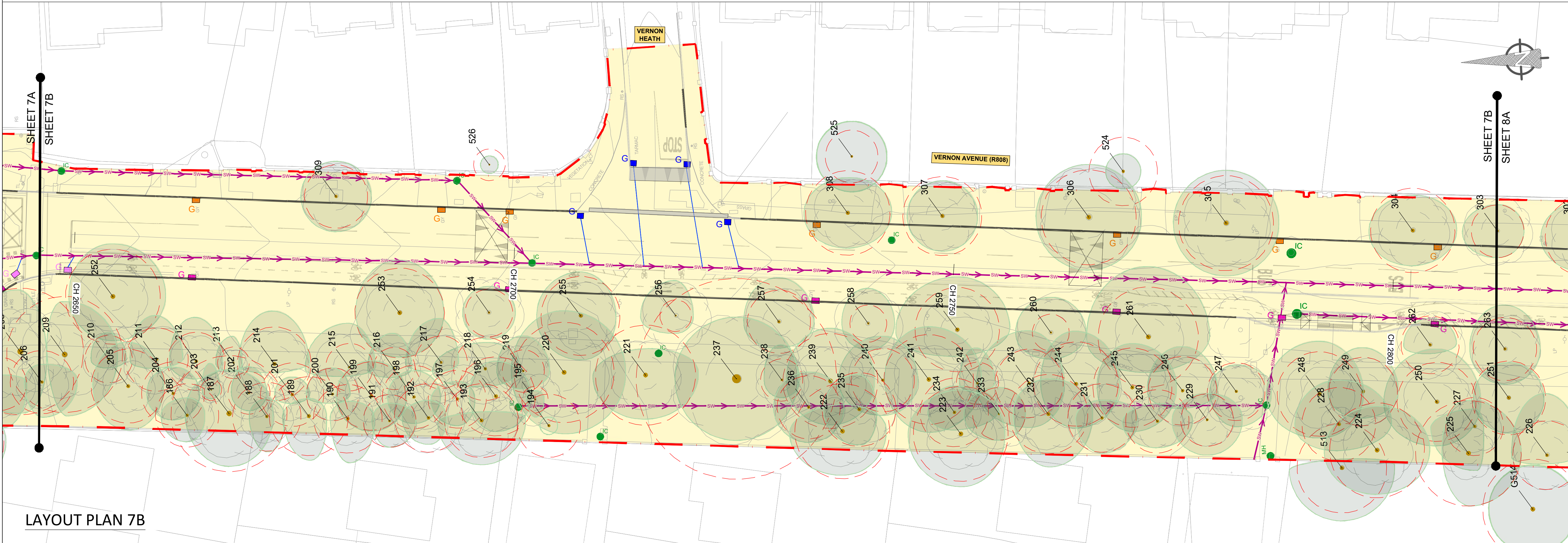
LAYOUT PLAN 7A
