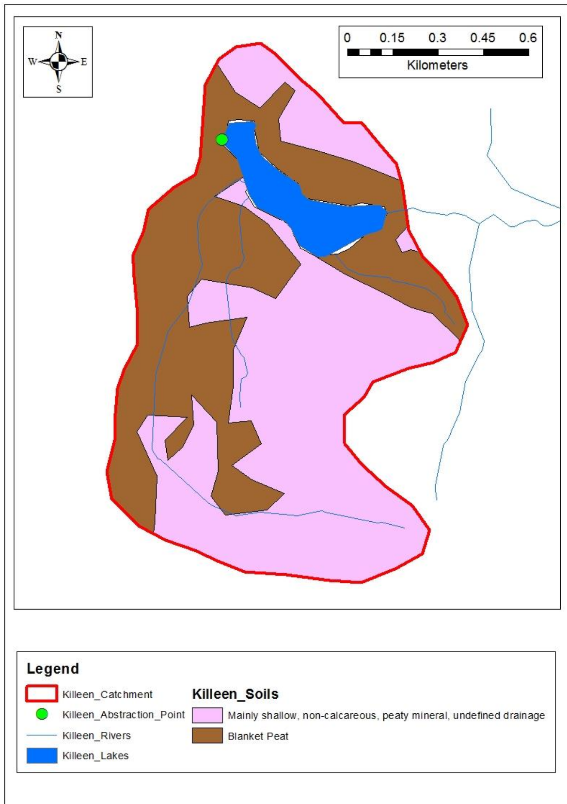
Figure 7: Soil types present within the Killeen GWS catchment.
