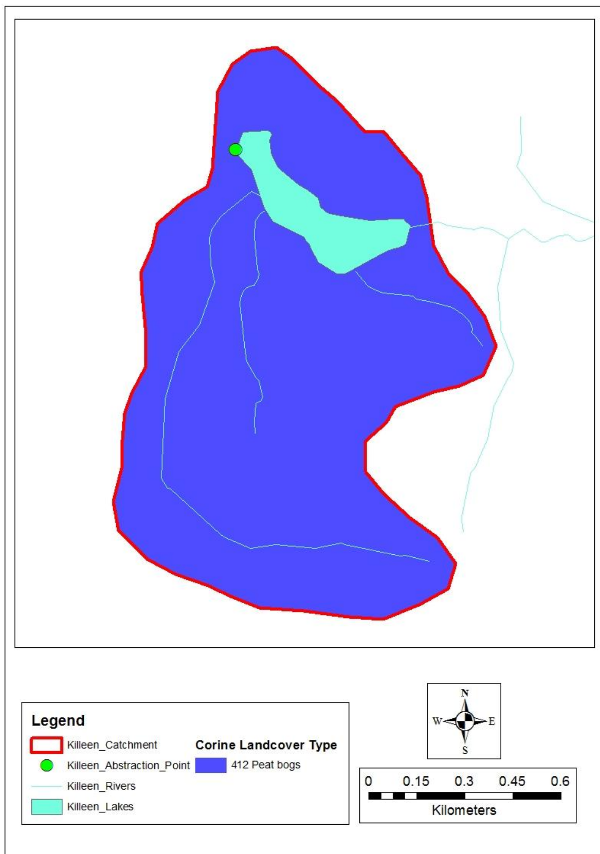
Figure 8: CORINE Land Cover classification within the Killeen GWS catchment.
