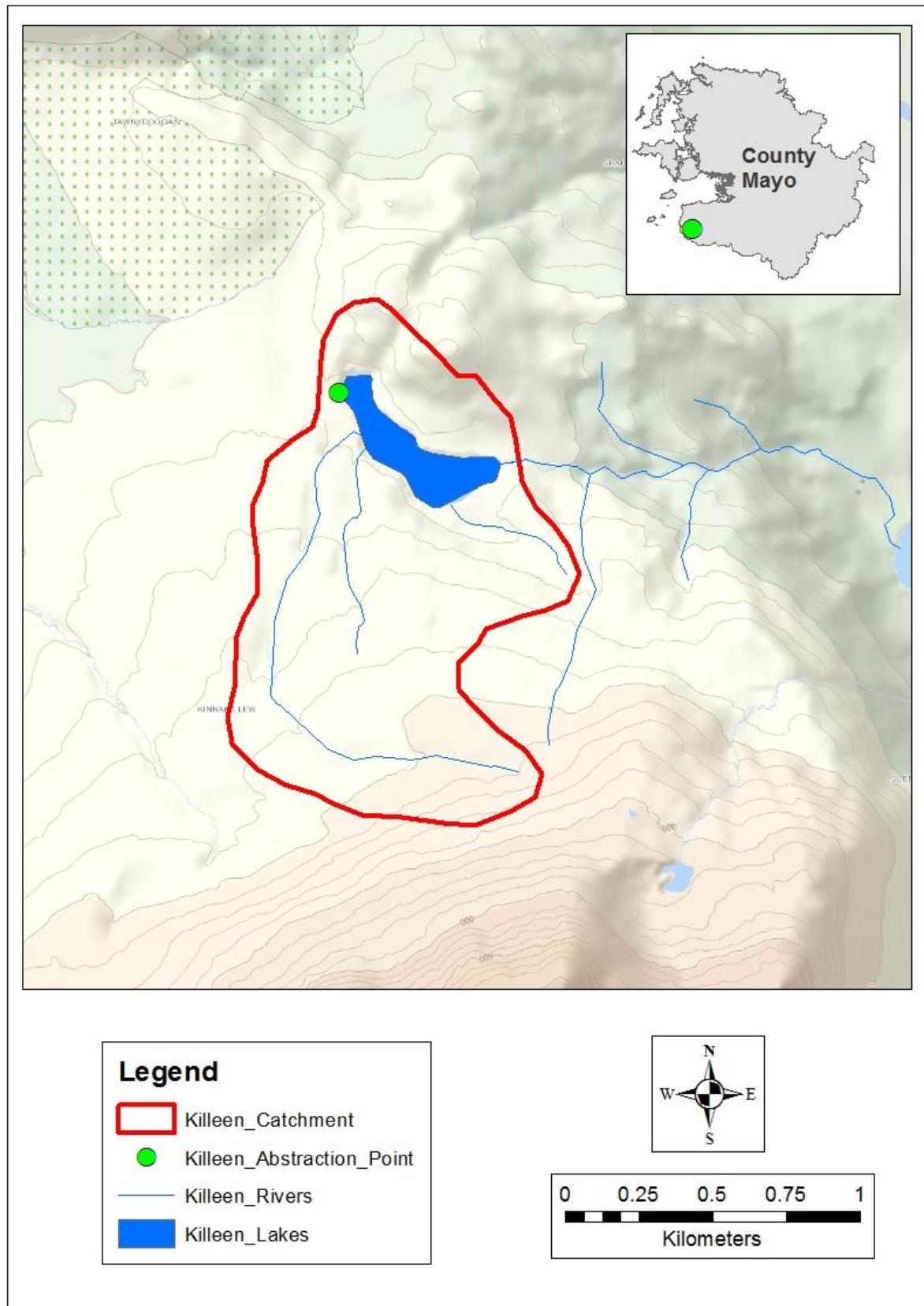
Figure 1: Surface water catchment area for the Killeen GWS.
