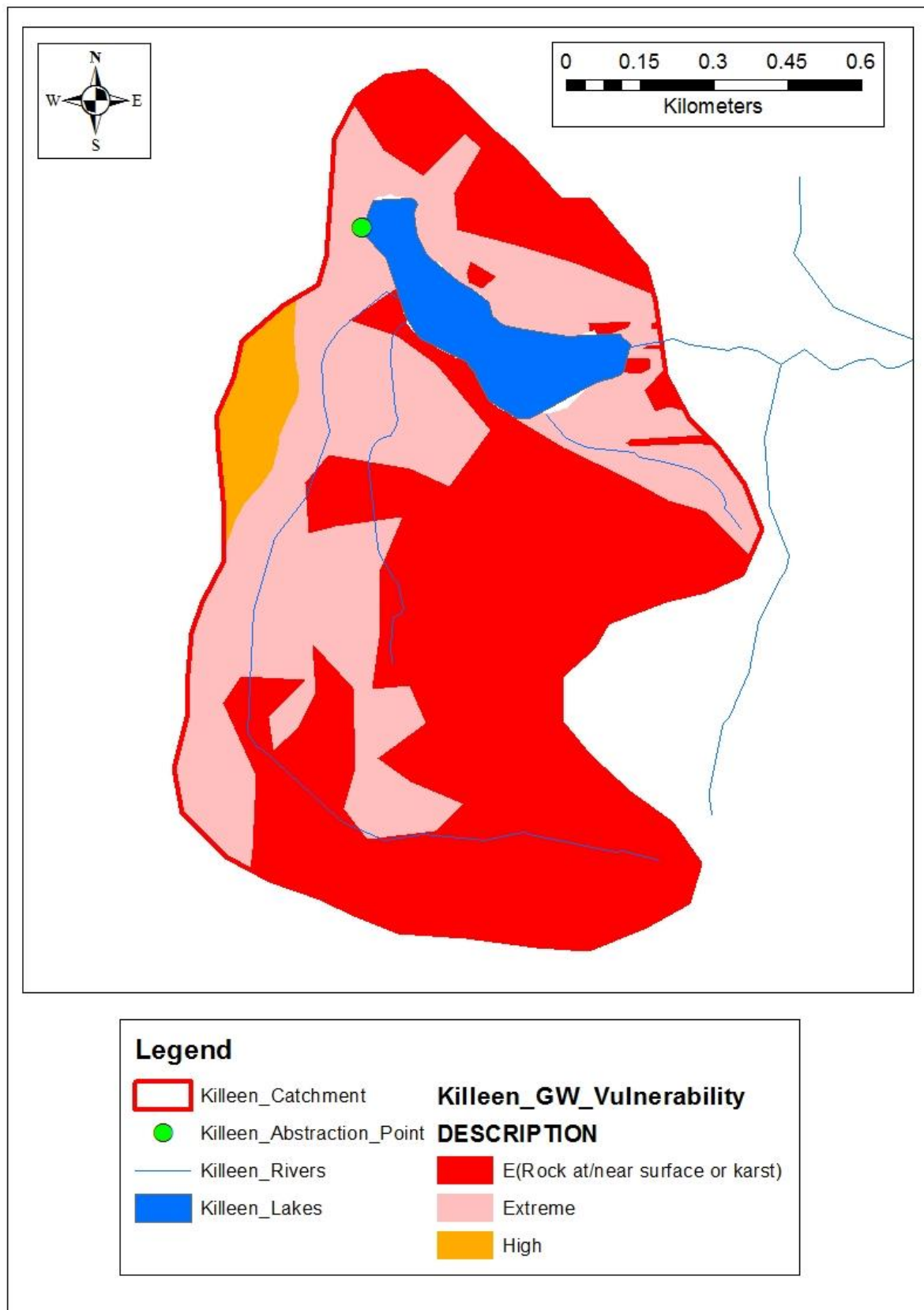
Figure 5: Groundwater vulnerability within the Killeen GWS catchment.
