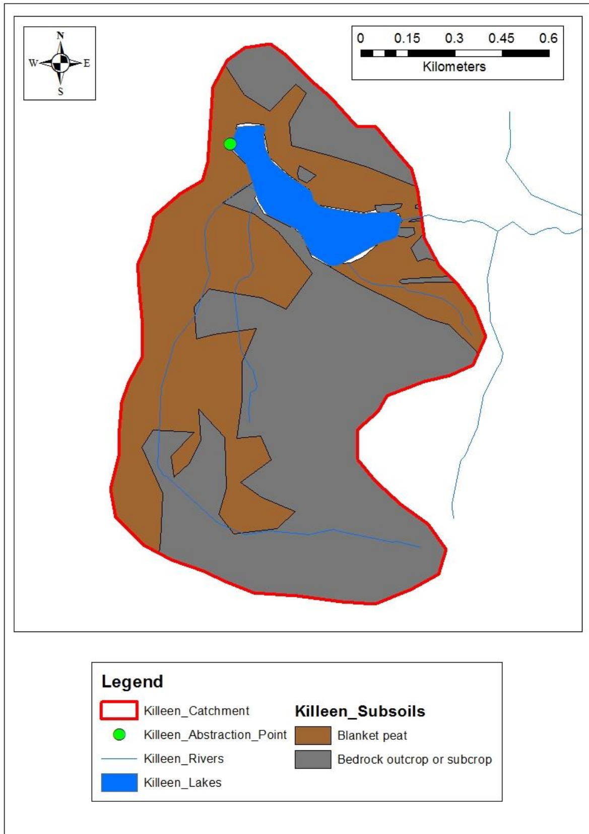
Figure 6: Subsoil deposits within the Killeen GWS catchment.
