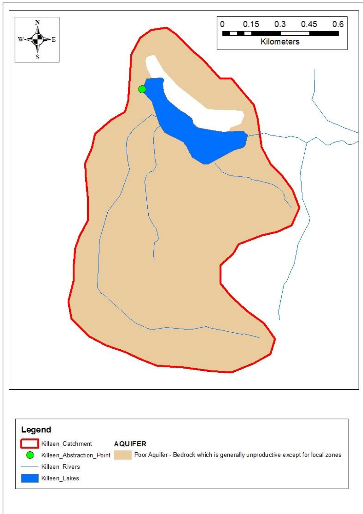
Figure 4: Aquifer types present within the Killeen GWS catchment.
