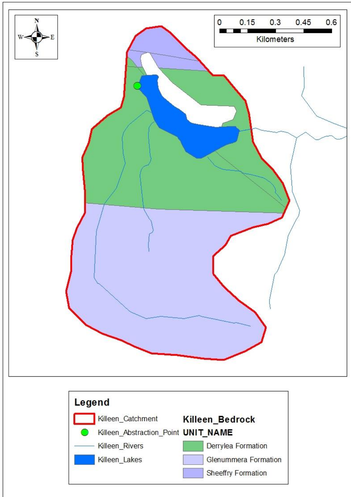
Figure 3: Bedrock geology within the Killeen GWS catchment.
