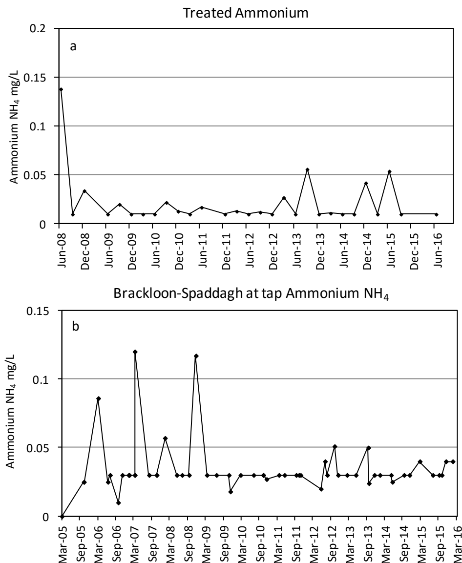
Figure 25: a) Treated water Ammonium concentration at Brackloon Spaddagh water treatment plant from June 2008 until June 2016 (date Source AECOM) and b) Treated water from Brackloon Spaddagh GWS March 2005 until February 2016. Data sources: Mayo County Council.
