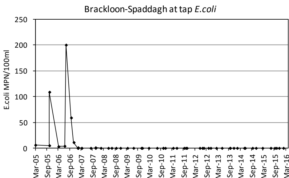
Figure 27: Treated water E. coli values at Brackloon Spaddagh GWS catchment from March 2005 until February 2016. Data source: Mayo County Council.
