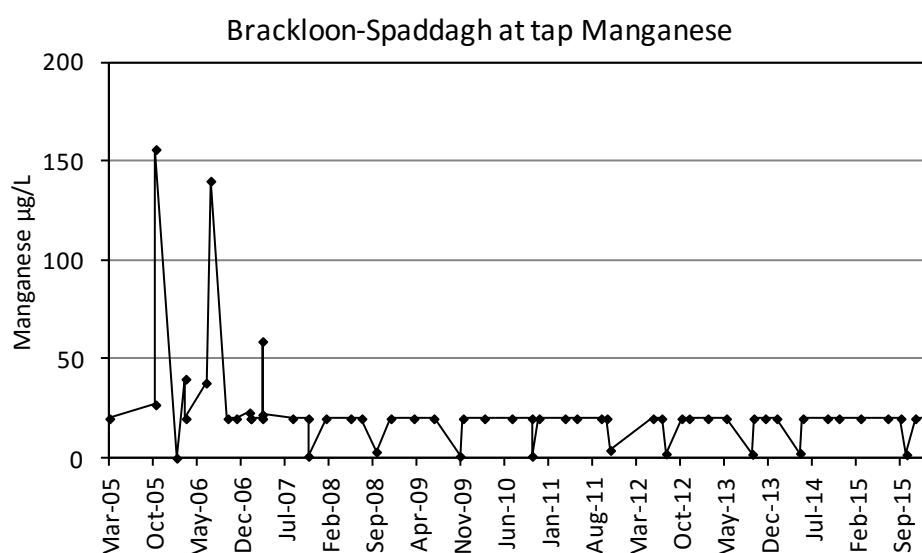
Figure 21: Manganese concentrations on treated water in the Brackloon Spaddagh GWS network from March 2005 until February 2016. Data source: Mayo County Council.
