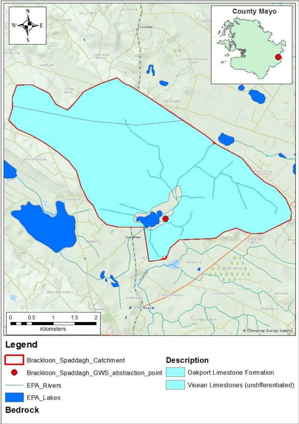
Figure 3: Bedrock geology within the Brackloon Spaddagh GWS catchment.
