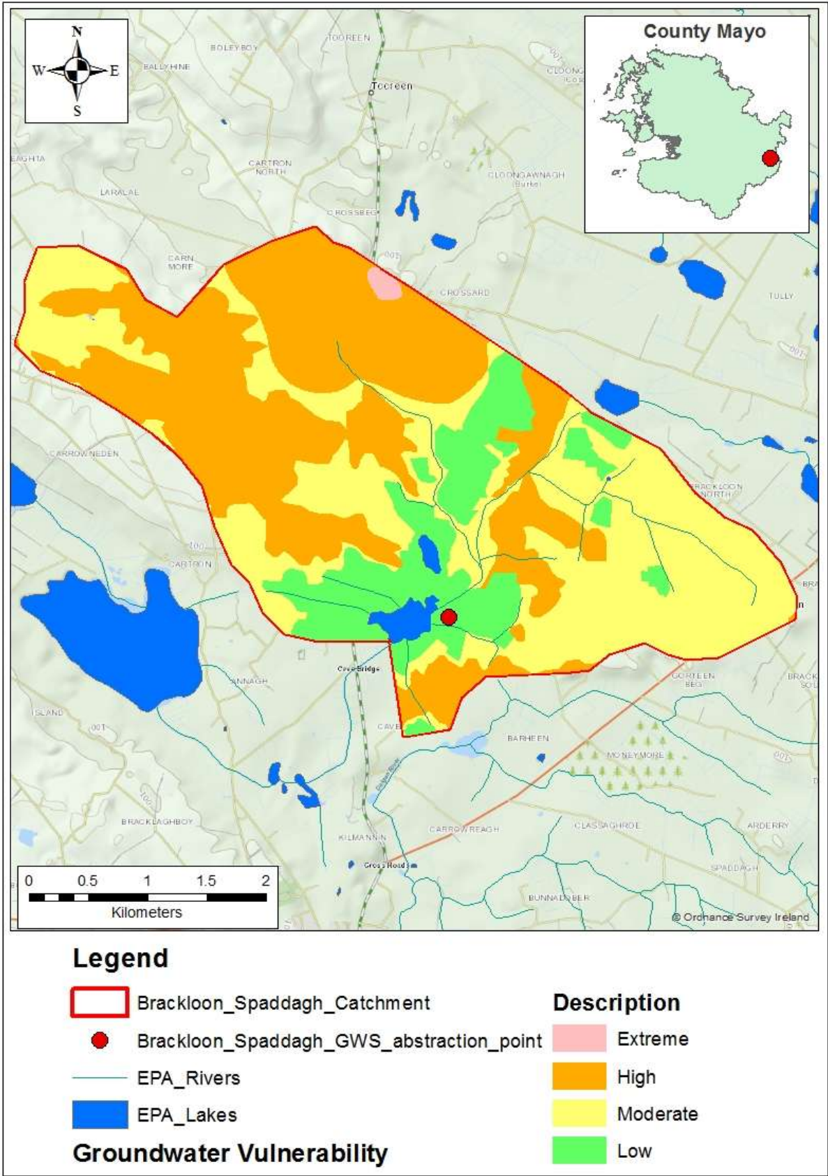
Figure 5: Groundwater vulnerability within the Brackloon Spaddagh GWS catchment.
