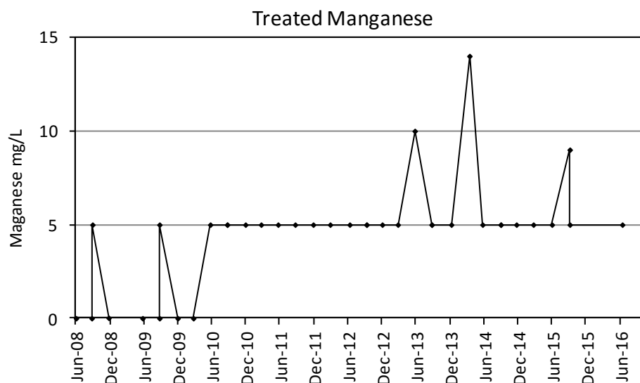
Figure 20: Treated water manganese concentrations at the Brackloon Spaddagh water treatment plant from June 2008 until June 2016. Data source: AECOM.
