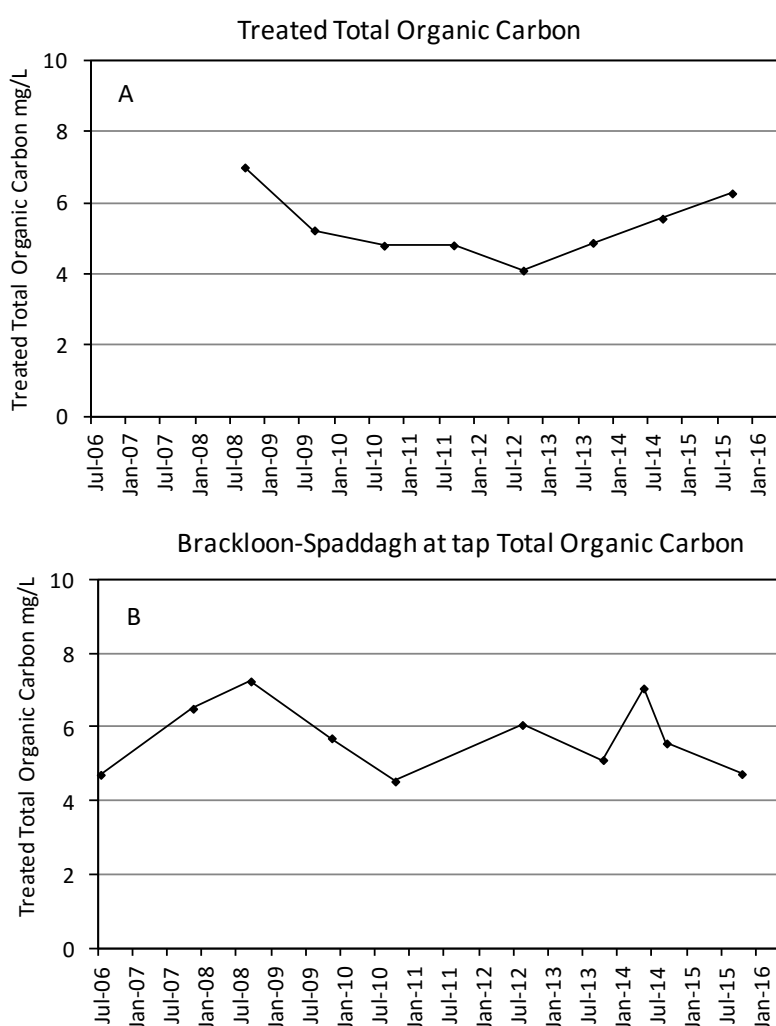
Figure 13: A) Total Organic Carbon from treated water at the Brackloon Spaddagh water treatment plant (data source AECOM) and B) Total Organic Carbon from treated water in the network from July 2006 until October 2015 (Data source Mayo County Council).
