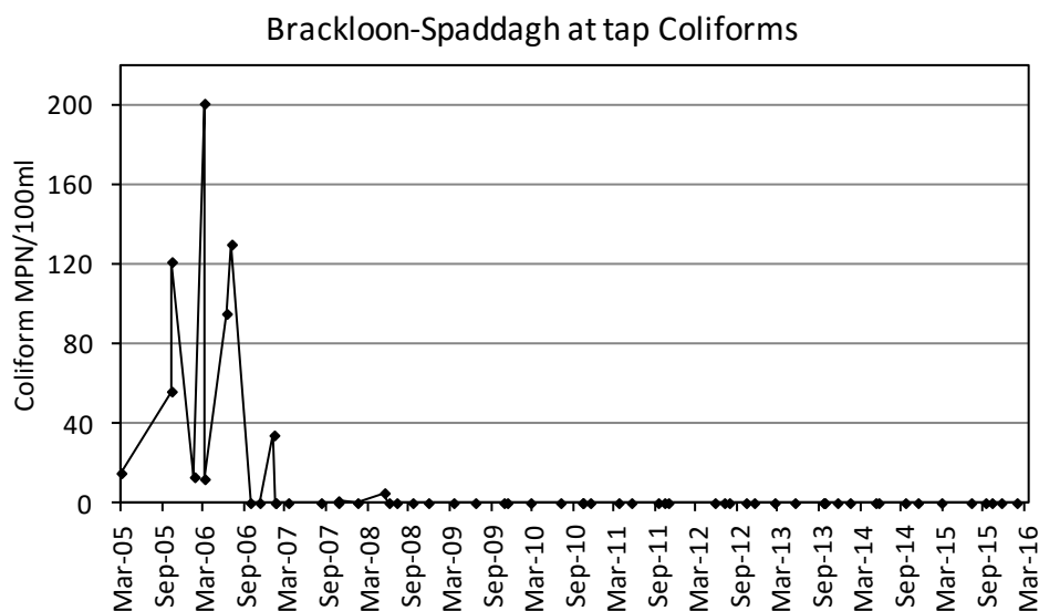
Figure 29: Treated water Coliforms from March 2005 until February 2016 from Brackloon Spaddagh GWS network. Data source: Mayo County Council
