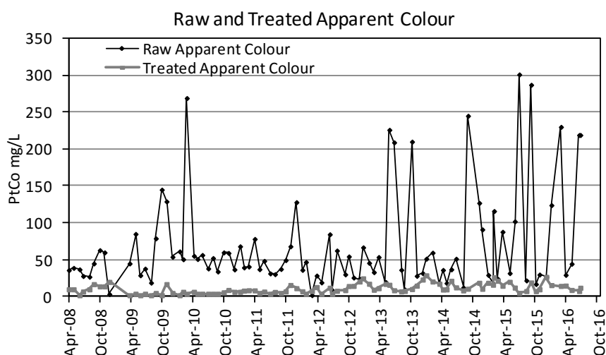
Figure 11: Raw and treated apparent water colour from Brackloon Spaddagh GWS water treatment plant from April 2008 until July 2016. Source data: AECOM and Glan Agua.
