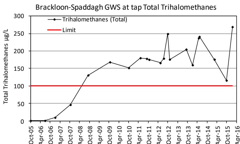
Figure 14: Total Trihalomethanes from treated water in the network from October 2005 until February 2016. Red line indicated the Drinking Water Regulations (2014) limit of 100 µg THM/L). Data source: Mayo County Council.
