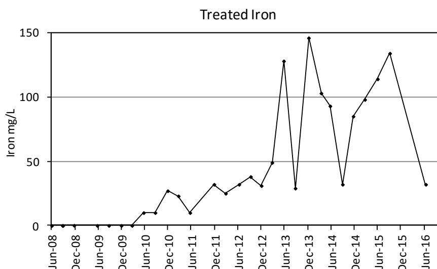
Figure 18: Treated water iron from Brackloon Spaddagh water treatment plant from June 2008 until July 2016. Data source: AECOM.
