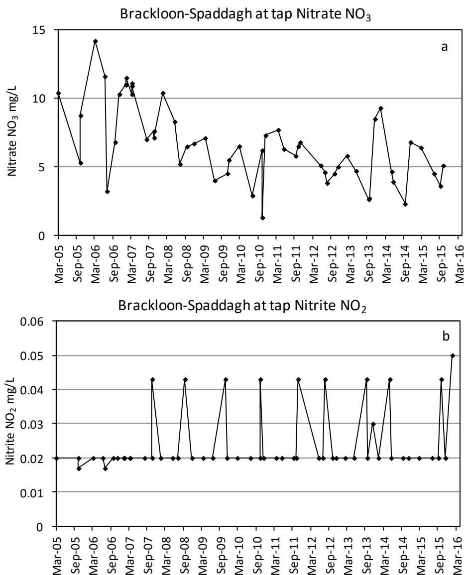
Figure 24: a) Treated water nitrate and b) treated water nitrites concentrations in Brackloon Spaddagh GWS network from March 2005 until February 2016. Data sources: Mayo County Council.
