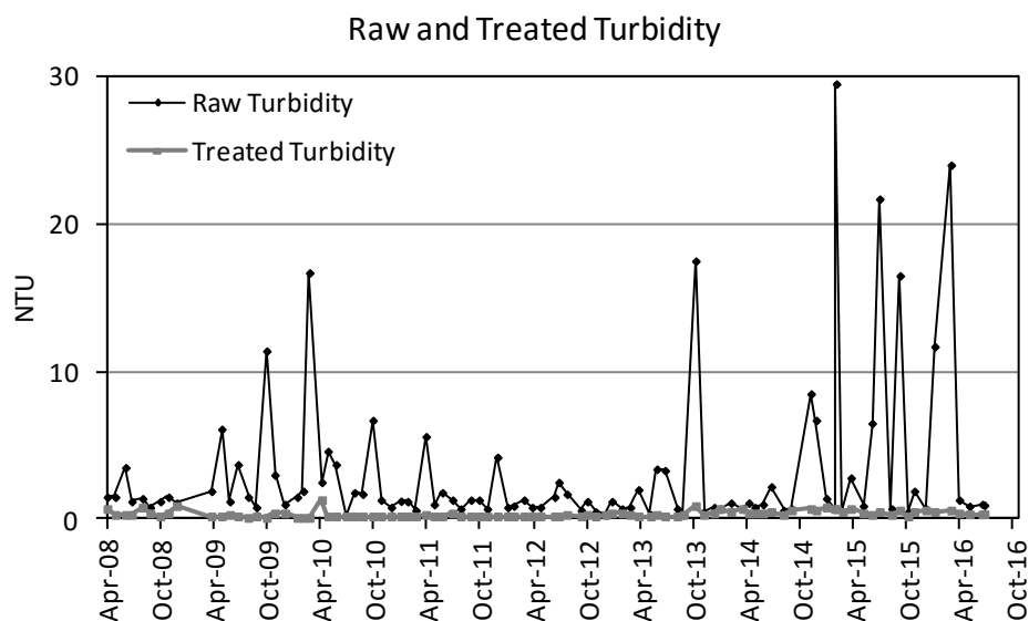
Figure 16: Raw and treated water turbidity from Brackloon Spaddagh water treatment plant from April 2008 until July 2016. Data source: AECOM and Glan Agua.
