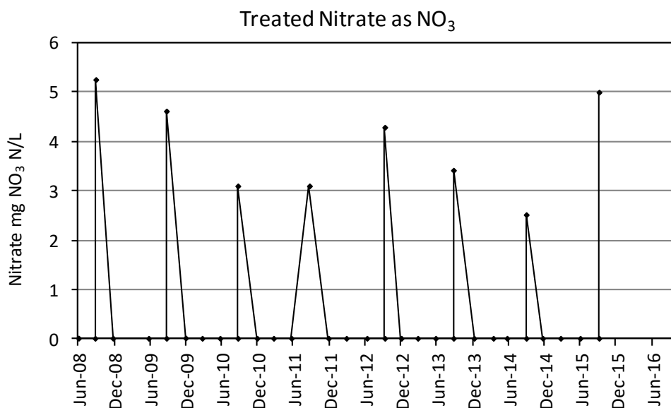
Figure 23: Treated water nitrate concentrations at Brackloon Spaddagh water treatment plant from June 2008 until September 2015. Data source: AECOM.
