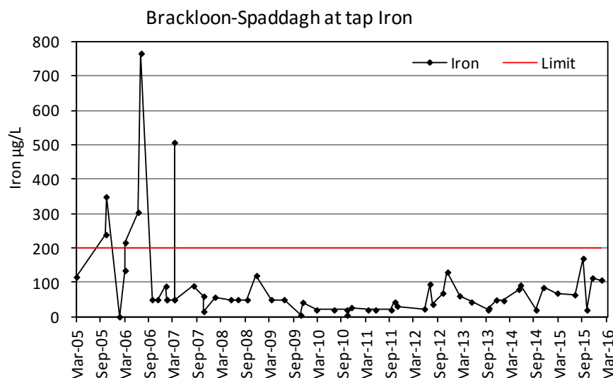
Figure 19: Treated water Iron concentrations in the network from March 2005 until February 2016. Data source: Mayo County Council.
