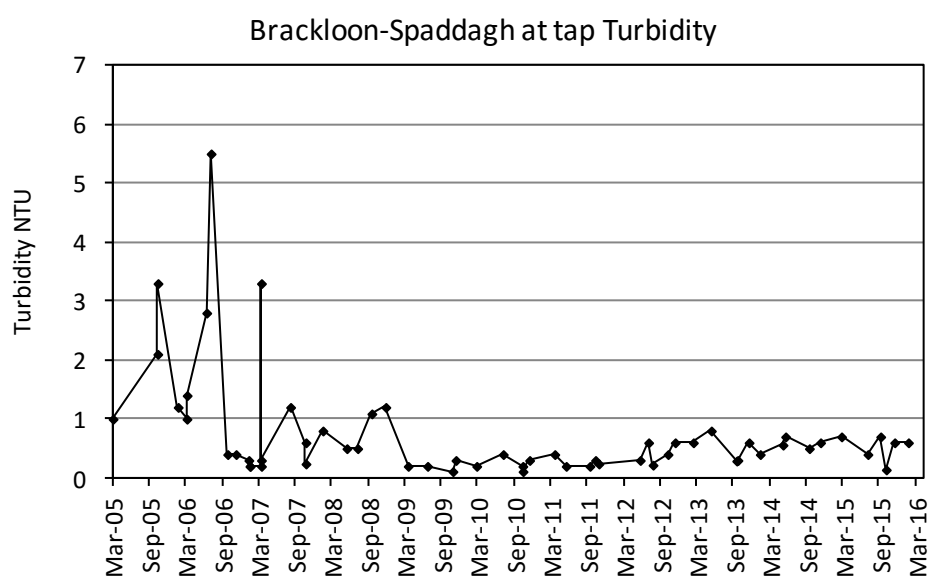
Figure 17: Treated water Turbidity at the tap from March 2005 until February 2016. Data source: Mayo County Council.
