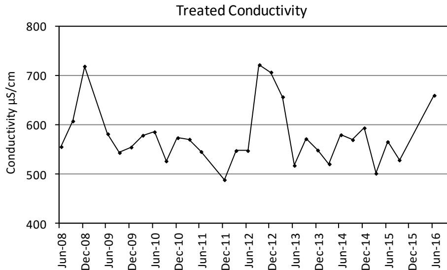
Figure 26: Treated water Conductivity from Brackloon Spaddagh water treatment plant from June 2008 until June 2016. Data source: AECOM and GlanAgua.
