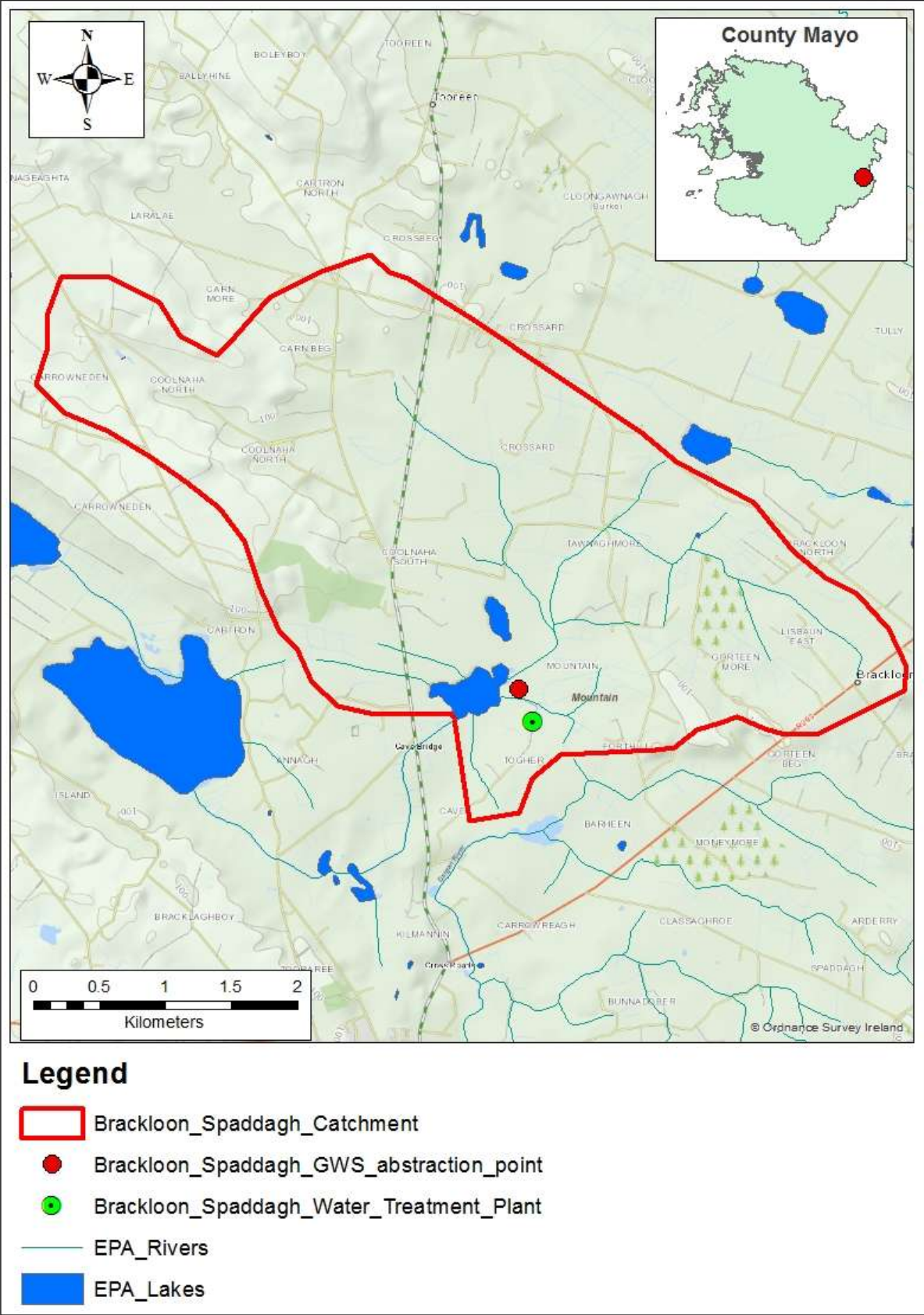
Figure 2: Catchment area and location of Brackloon Spaddagh GWS abstraction point and water treatment plant.
