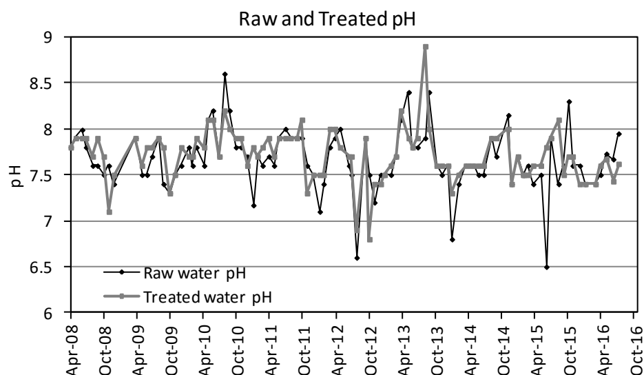
Figure 22: Raw and treated water pH levels at Brackloon Spaddagh water treatment plant from April 2008 until July 2016. Data source: AECOM and Glan Agua.
