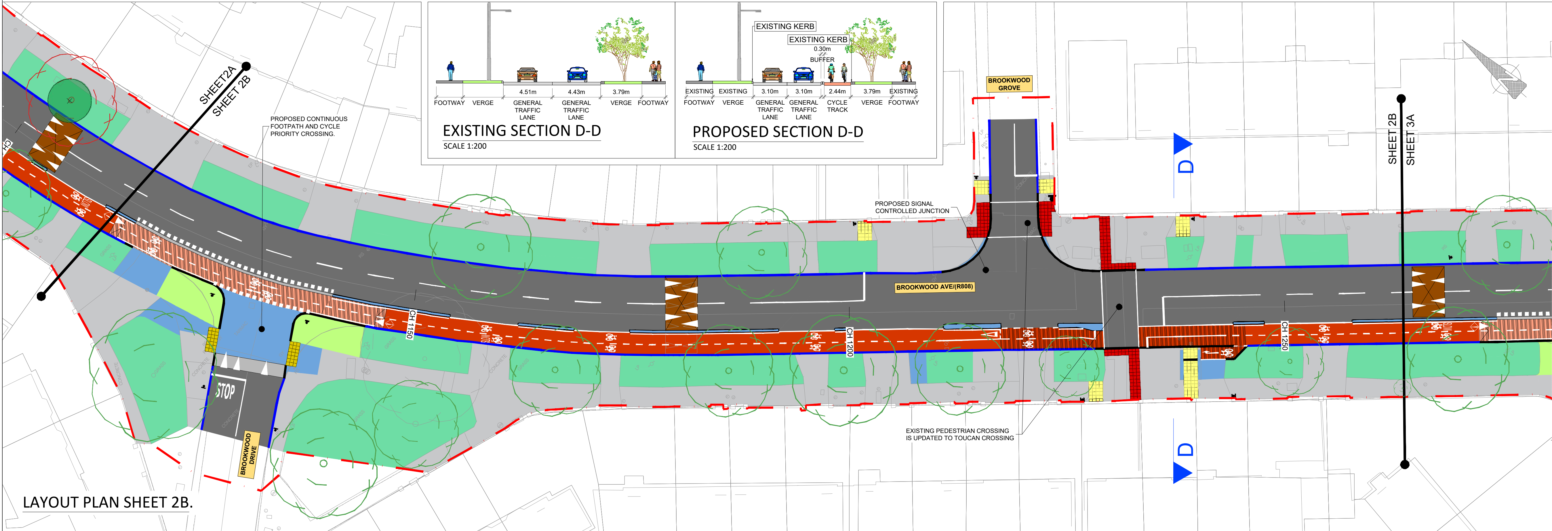
LAYOUT PLAN SHEET 2A.
