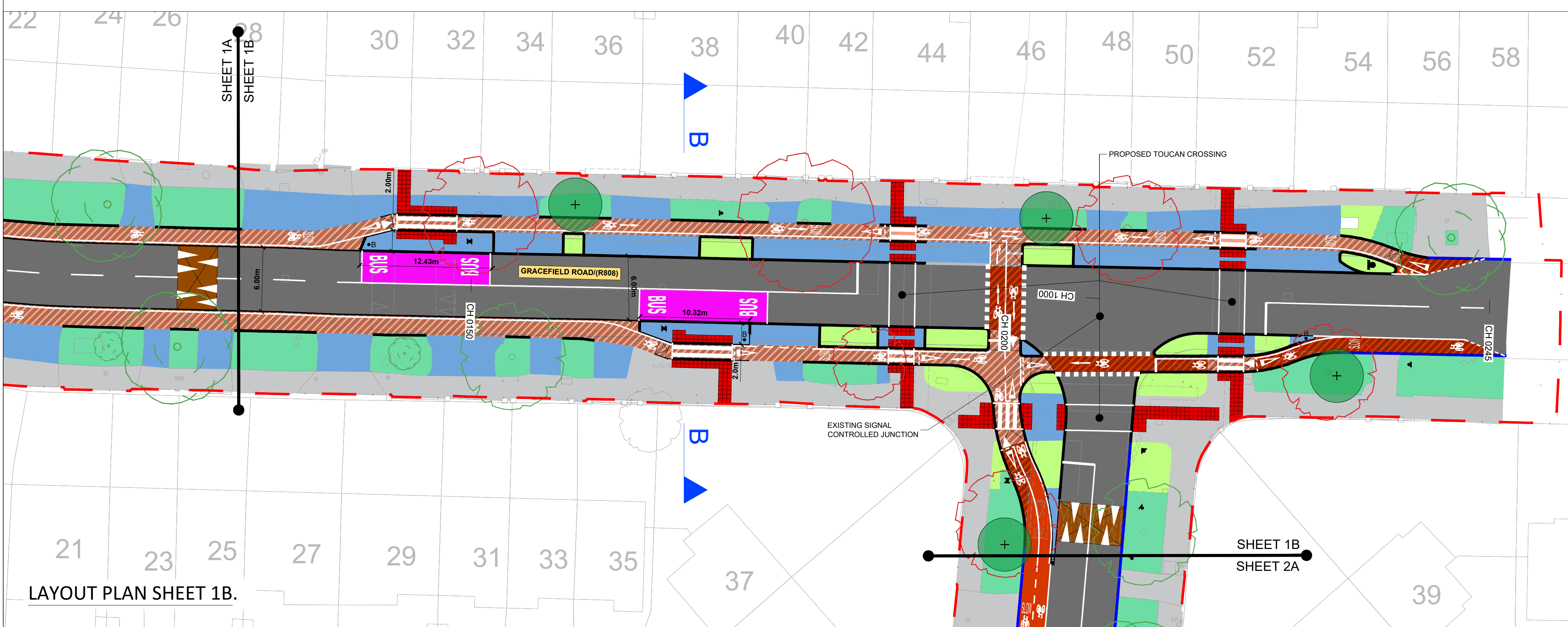
LAYOUT PLAN SHEET 1A.
