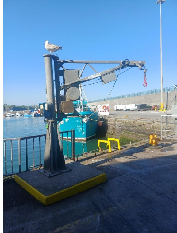
Lifting Davit
