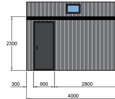
Side Elevation Scale 1:100
