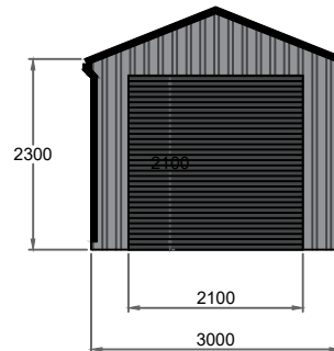
Front Elevation Scale 1:100
